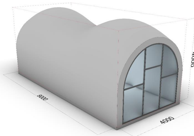
Fig 2 -Artistic Impression of final Volumetric Concrete Pod (For reference)
