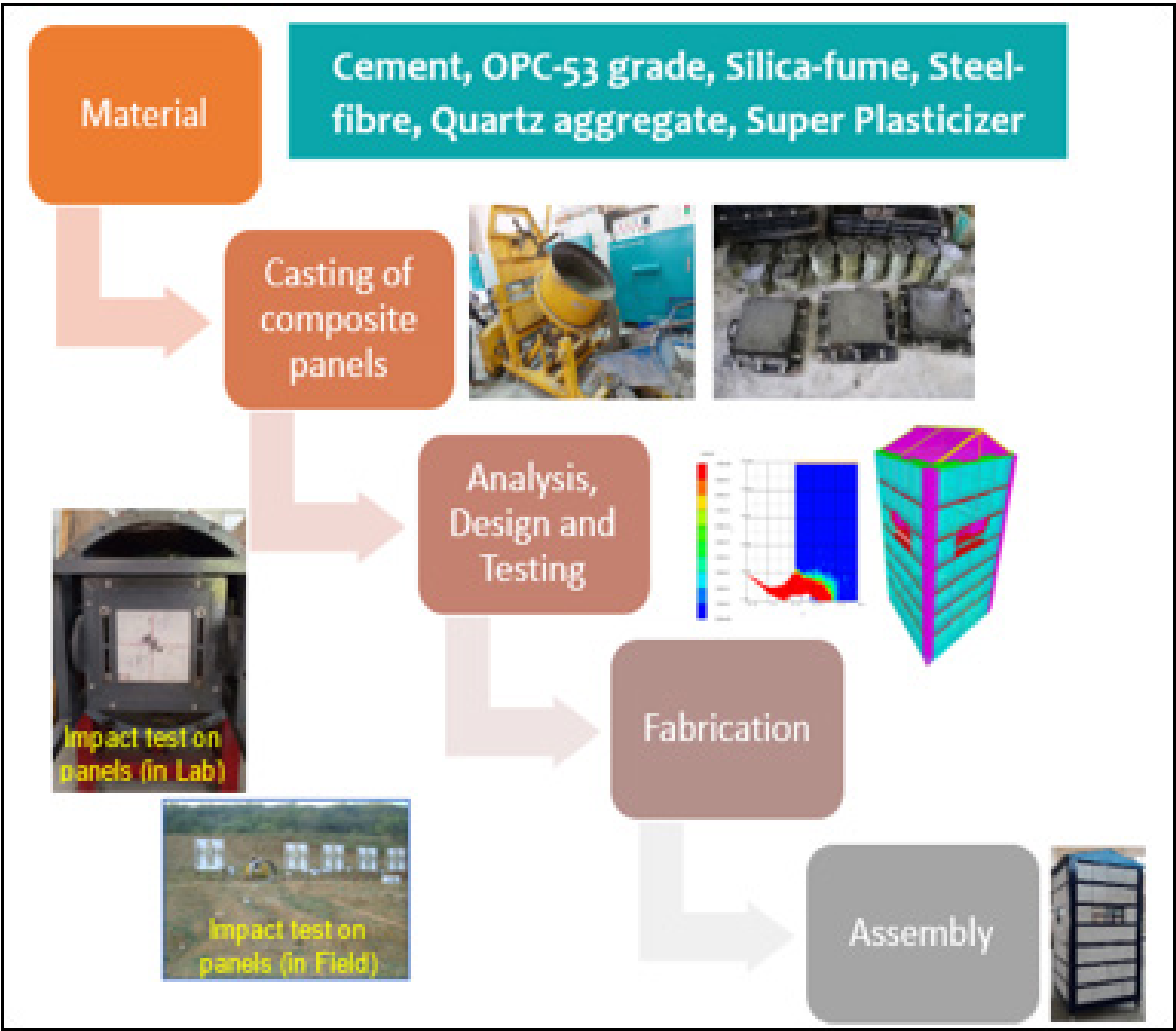
Methodology of multi hit resistant movable security booth development
